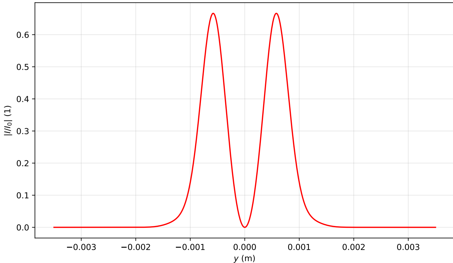
Intensity profile I(x=0, y, z=0.955)/I_0 , P_{in}=2.0P_{cr} , artificial time
